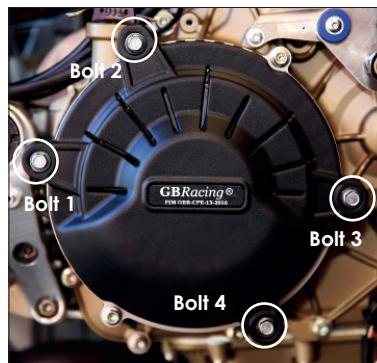
FIG 5. GBRacing cover fitted directly over the dry clutch - REUSE OE BOLTS
